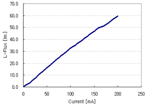
Current vs. L-Flux
