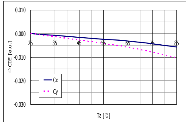
(4) CIE x , Δ CIE y vs. Temperature
