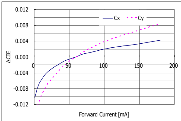
(3) CIE x , Δ CIE y vs. Forward Current
