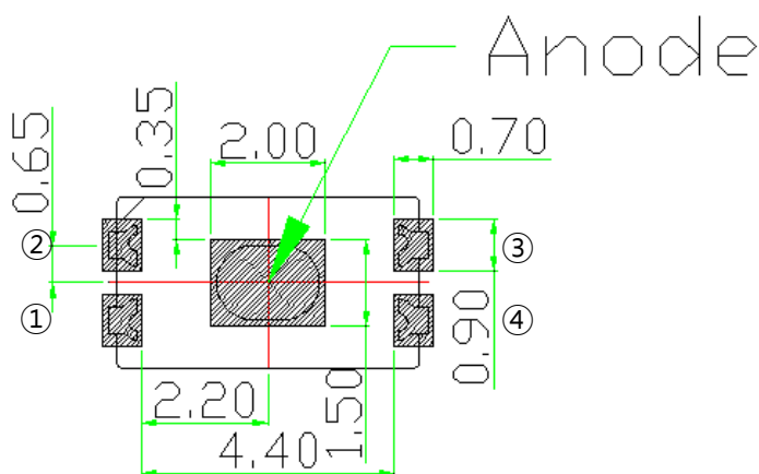
Solder Land
