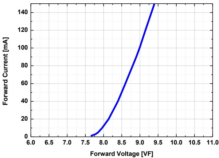
(1) Forward Voltage vs Forward Current
