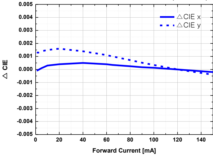
(5) Relative Chromaticity Coordinate vs Forward Current ( T_a = 25^\circ\text{C} )
