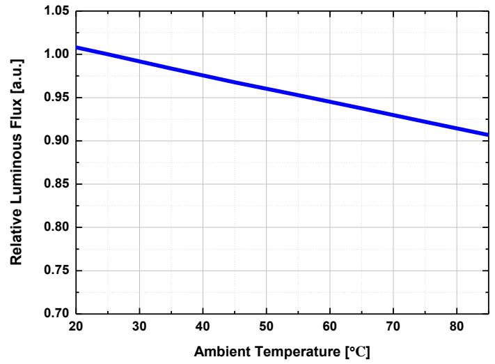
(4) Relative Luminous Flux vs Ambient Temperature ( T_a = 25^\circ\text{C} )
