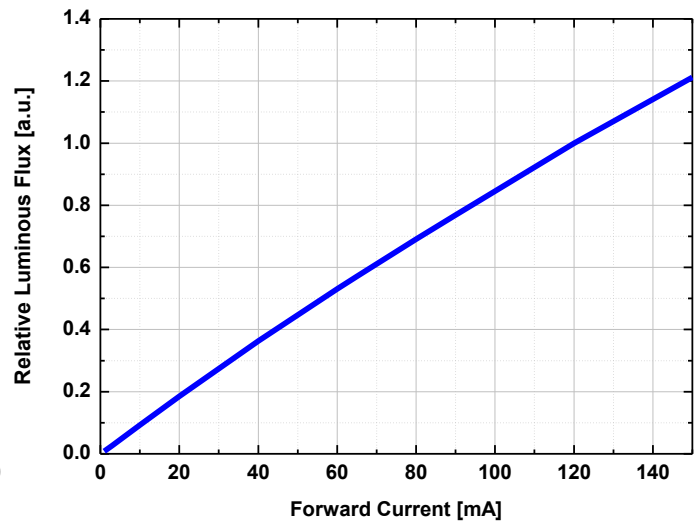
(2) Forward Current vs Relative L-Flux
