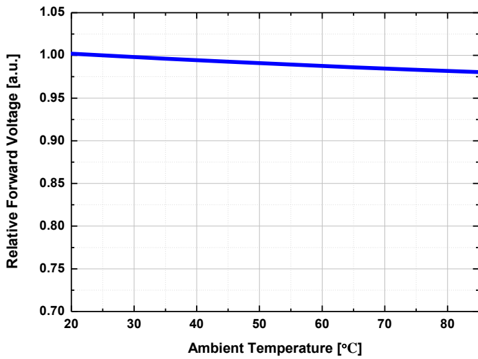
(3) Relative Forward Voltage vs Ambient Temperature ( I_F = 120\text{mA} )
