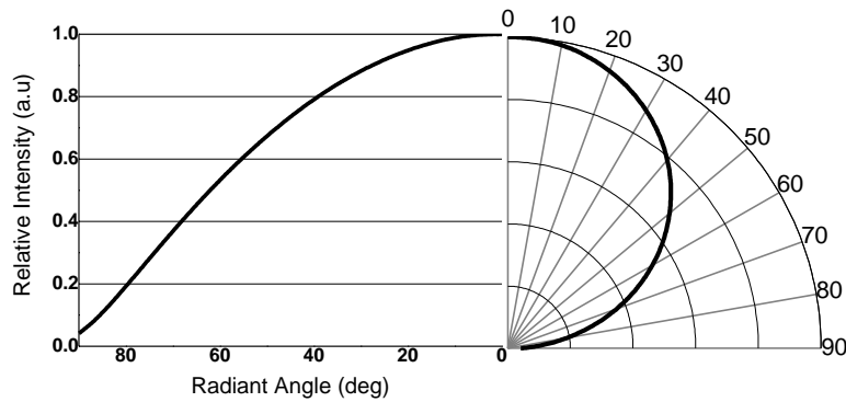
(5) View angle profile
