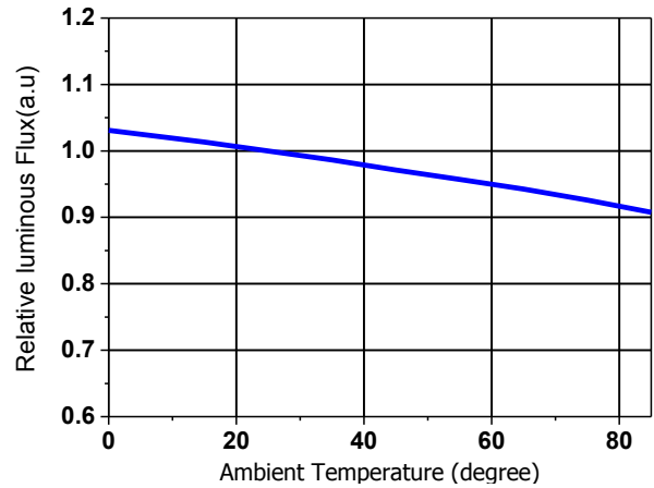
(4) Ambient Temperature vs Relative L-Flux
