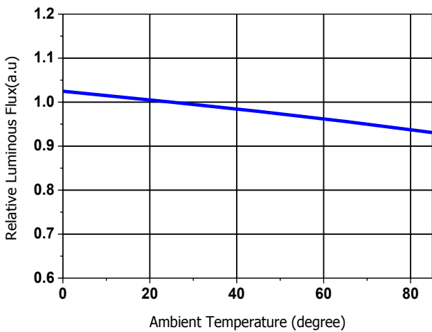
(5) Relative Luminous Flux vs Ambient Temperature
